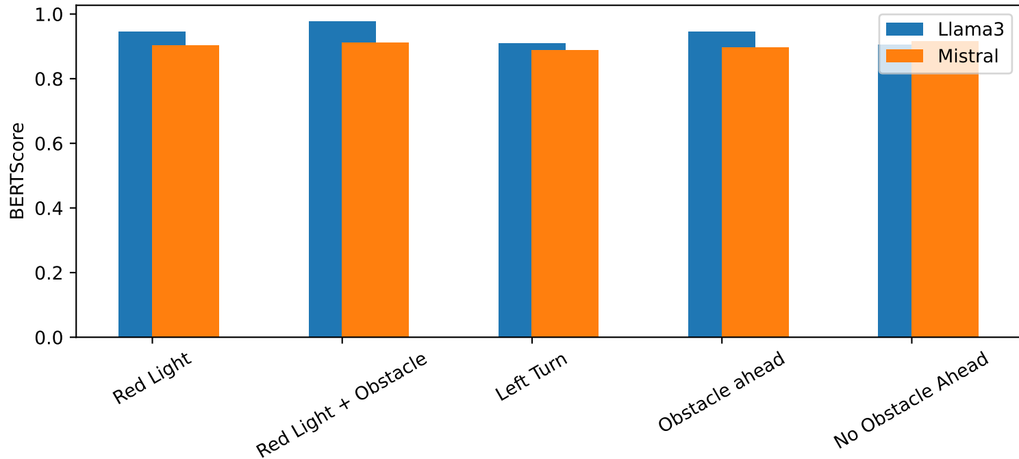
BERTScore Comparison by Scenario
